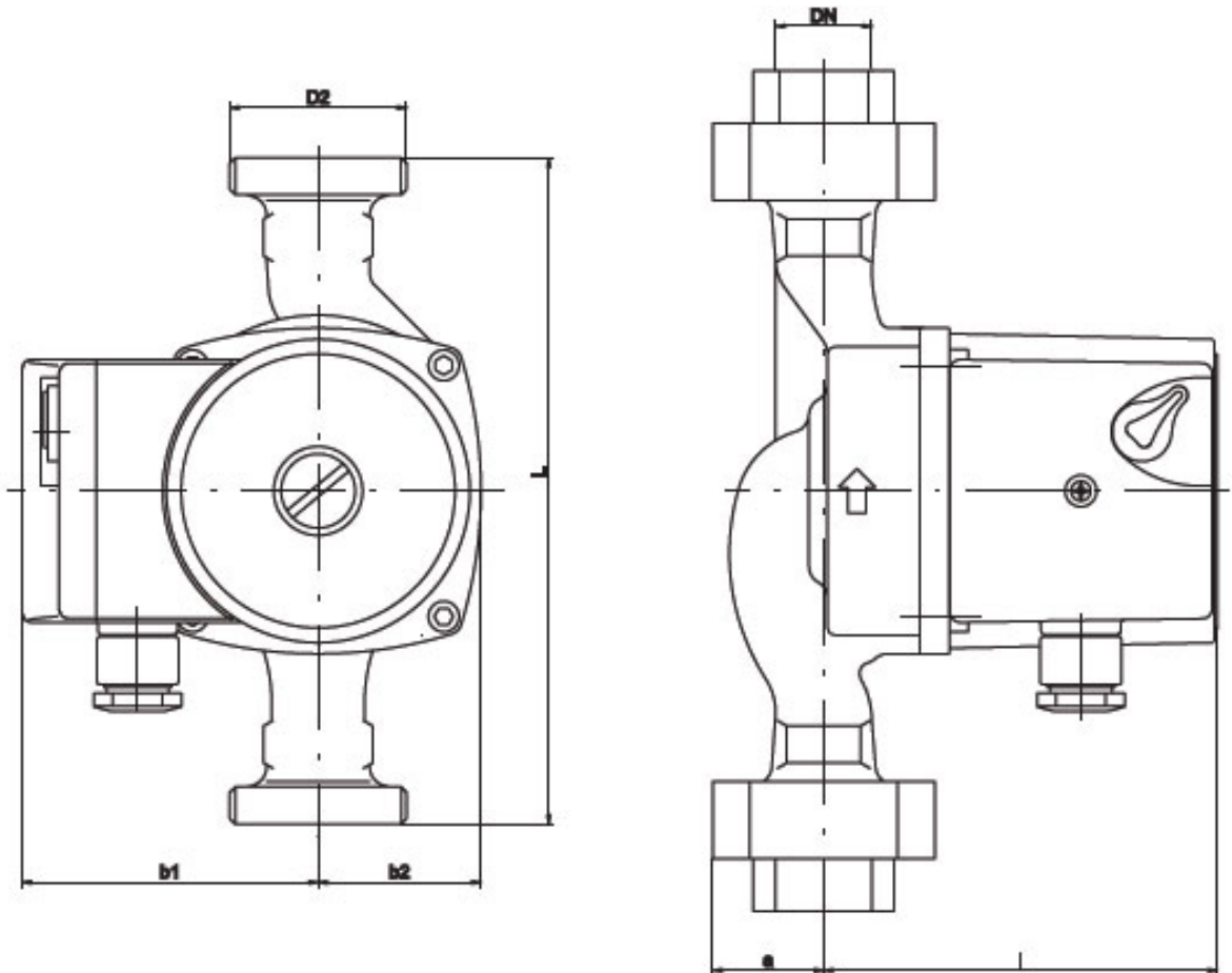
Dimension drawing
